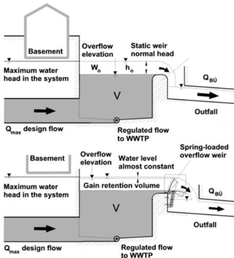
Figure 1: Demonstration of the efficiency of the HYDROVEX® Flap Spring-loaded Weir compared to a static weir
