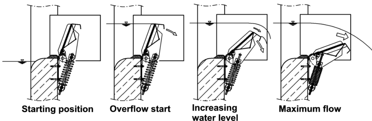
Figure 3 : Various operating phases of the spring overflow
