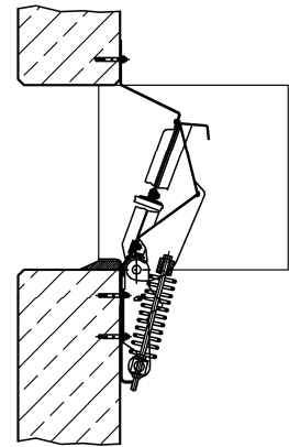
Figure 4: Use of HYDROVEX® Flap Spring-loaded Weir as backwash device
