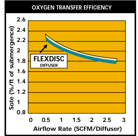
This chart demonstrates the superior oxygen transfer efficiency provided by FlexDisc fine bubble diffusers.
